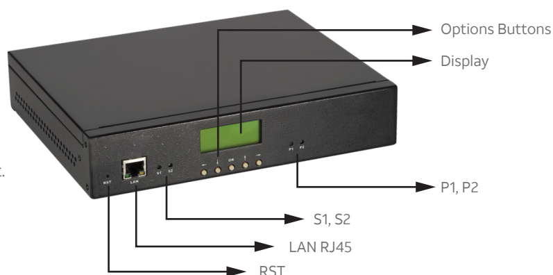
Front View of Channel Infrastructure Analyzer
